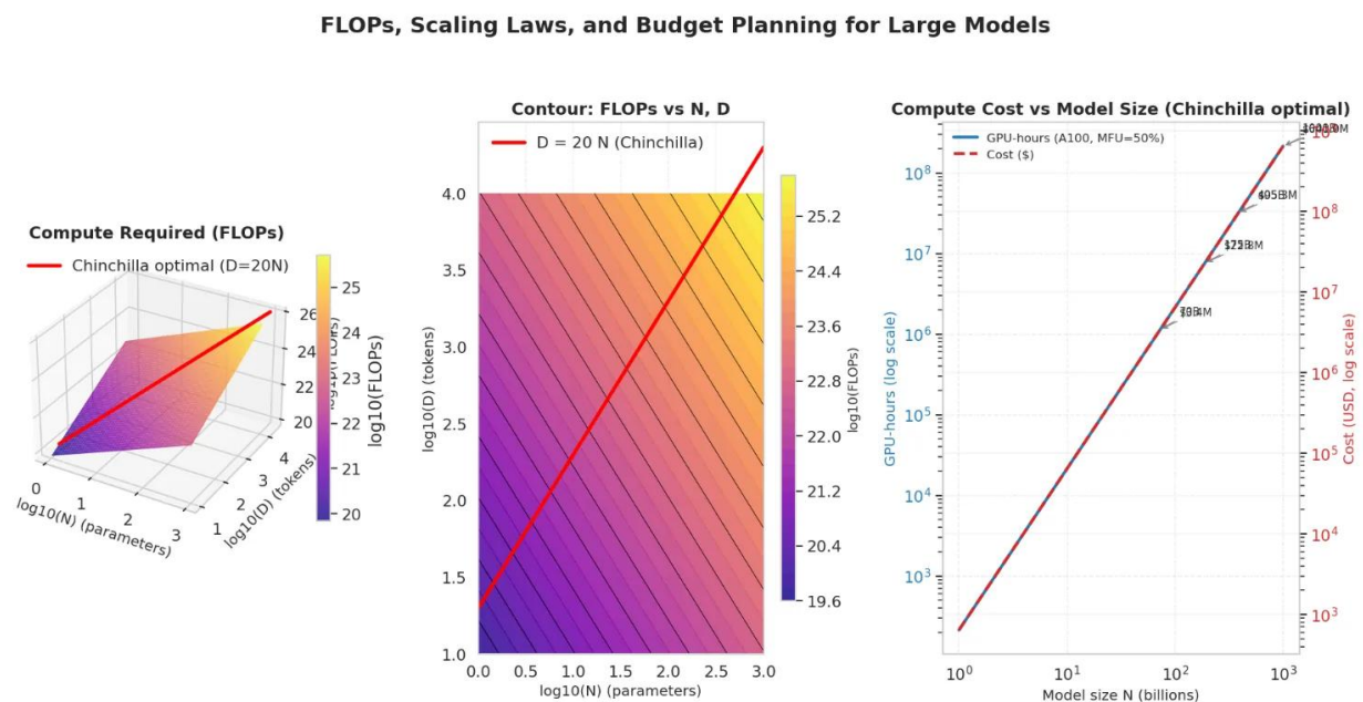
Figure 9: FLOPs and cost estimation for dense Transformer training.
