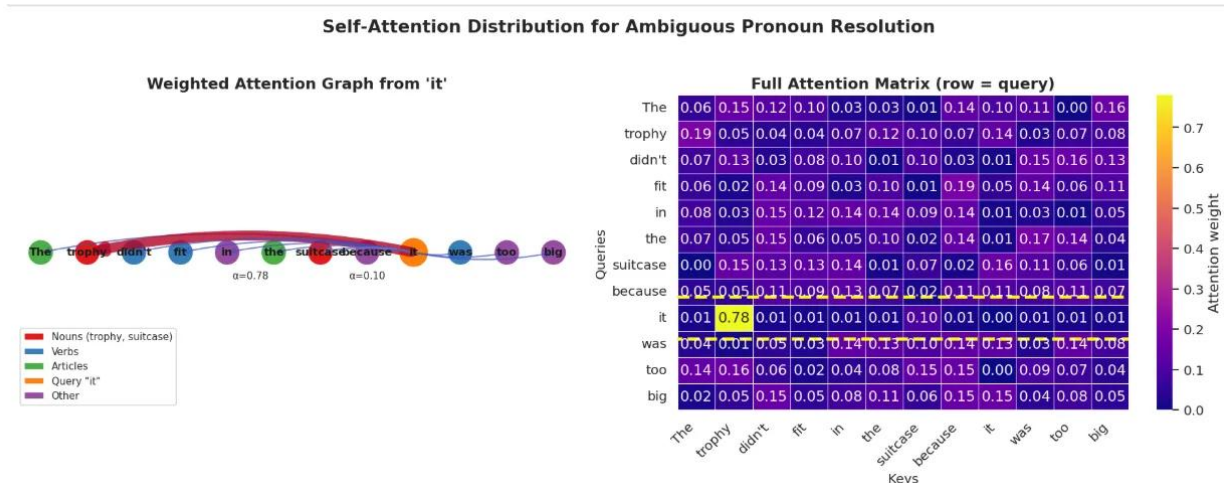
Figure 8 : Attention visualisation for the Winograd-style sentence "The trophy didn't fit in the suitcase because it was too big."
